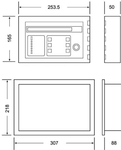
Bezel cutout - 267 x 179 x 90 All dimensions in mm.
