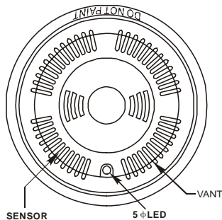
Figure 4 Front cover of detector head
